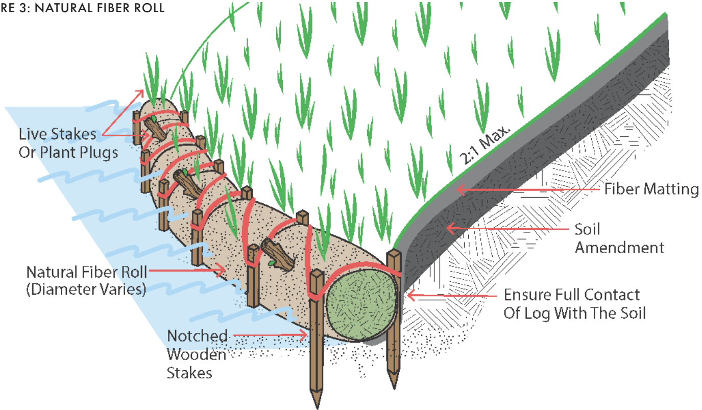
FIGURE 3: NATURAL FIBER ROLL
